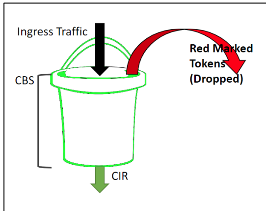
Figure 5-23 Two-color marker
