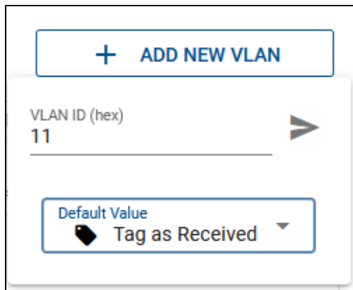
Figure 5-19 Egress VID remarking
