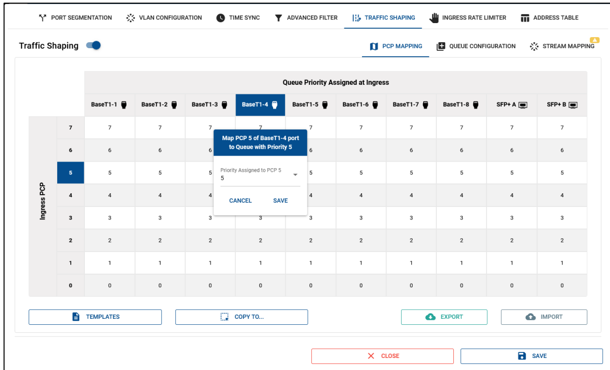
Figure 5-21 Traffic Shaping. PCP Mapping View
