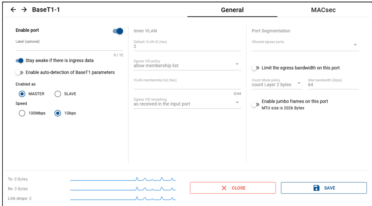
Figure 5-6 Configuration Menu for BASET-1 Port
