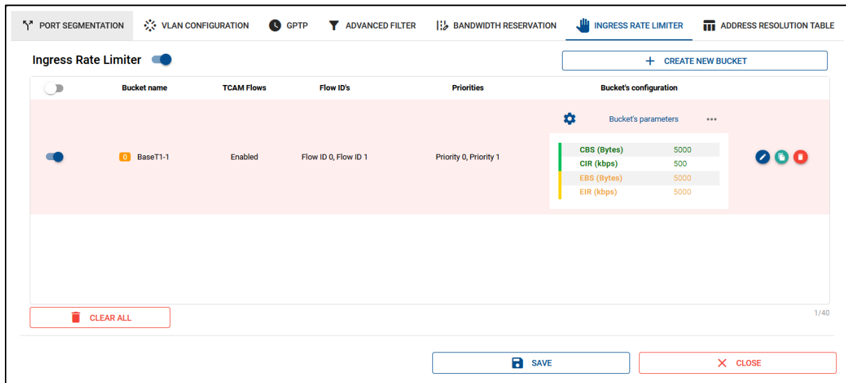
Figure 5-27 Ingress rate limiter
