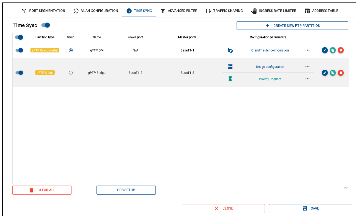
Figure 5-24 TimeSync configuration
