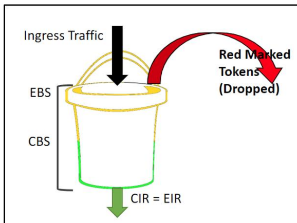
Figure 5-29 Three color single rate
