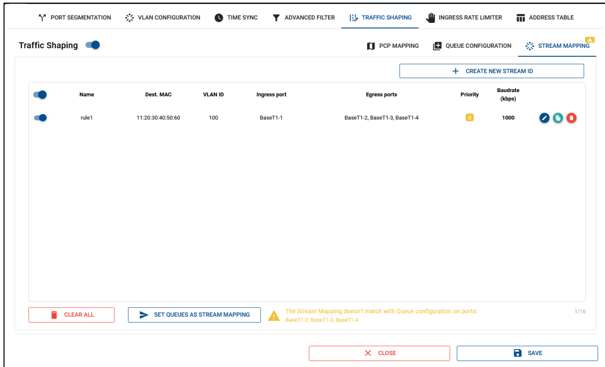
Figure 5-22 Traffic Shaping. Stream Mapping view.
