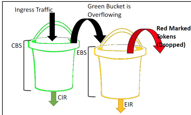
Figure 5-30 Three color double rate
