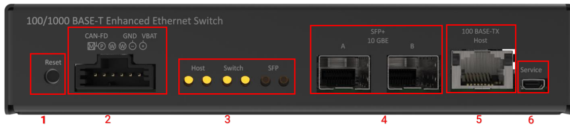
Figure 4-1: Front side of Enhanced Ethernet Switch
