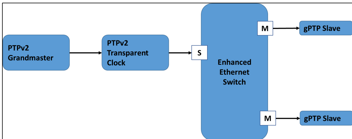
Figure 5-26 PTPv2 to gPTP Bridge
